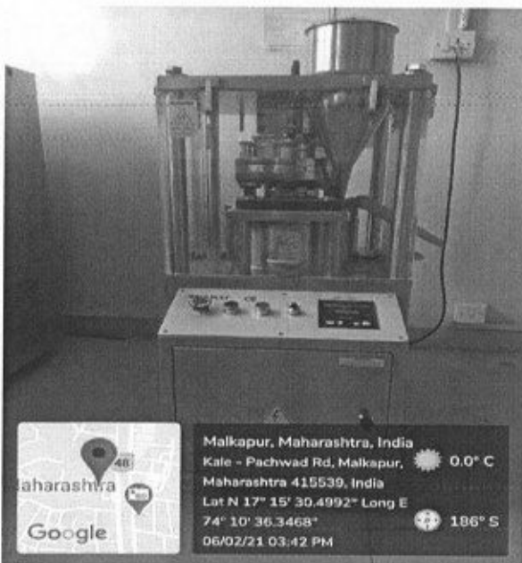
Rotary Tablet Press
